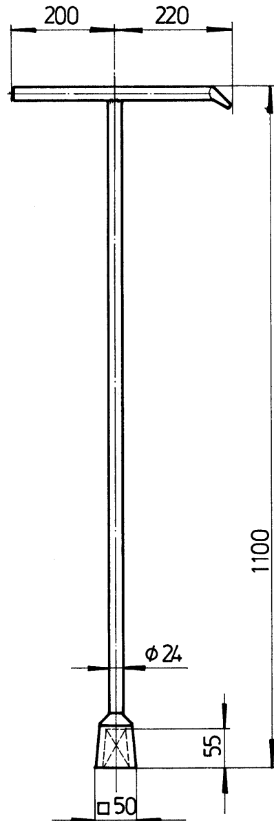
Bedienschlüssel 4-kt. DIN 3223
